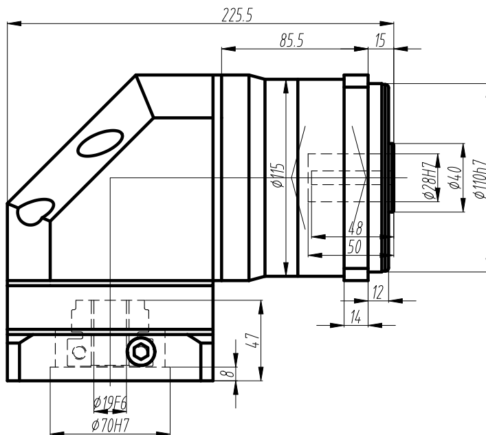
标准轴 Standard output shaft
